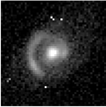
Euclid-like VIS
