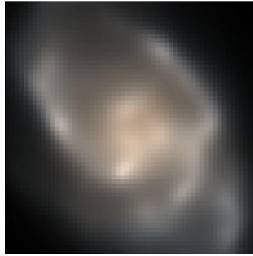
SR composite
