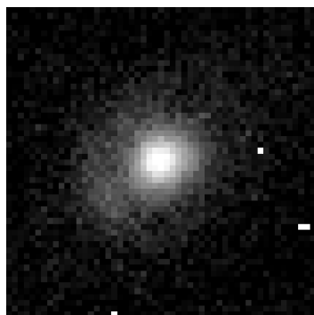
Euclid-like H E
