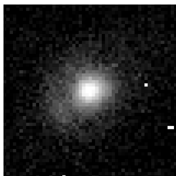
Euclid-like H_E
