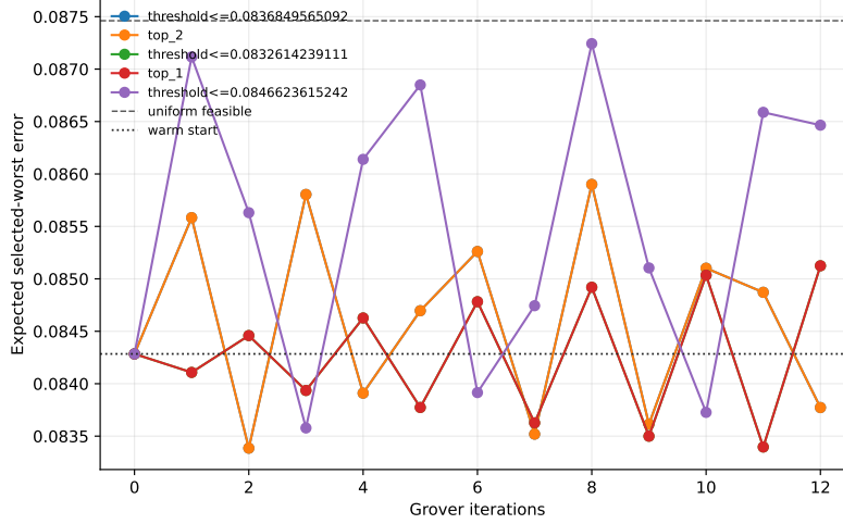
Figure 1: Warm-started one-coast Grover sweep used as an exploratory diagnostic. The predeclared protocol uses the top-2 oracle and the fixed iteration rule rather than choosing this curve after the sweep.
