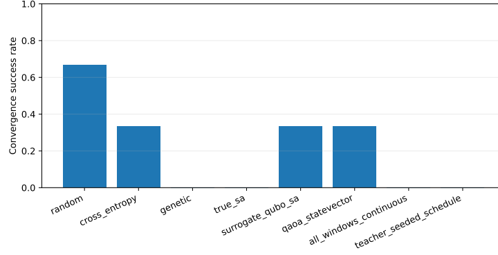
Figure 4: Teacher-controlled selected-branch refinement success rates. The result demonstrates nonzero recovery success but not quantum advantage.
