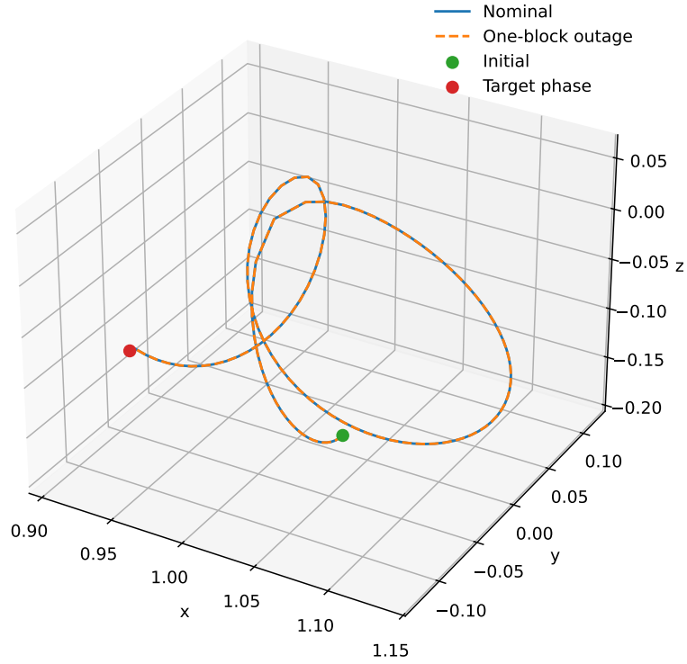
Figure 3: Example trajectory from the teacher-controlled benchmark. The case is a normalized CR3BP algorithm benchmark, not a flight-ready trajectory.
