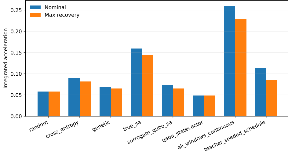
Figure 2: Teacher-controlled nominal and recovery fuel summaries. Fuel differences must be interpreted together with feasibility and missed-thrust error.
