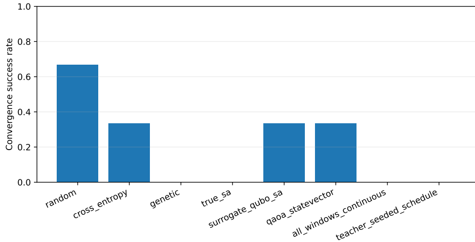
Figure 1: Teacher-controlled selected-branch refinement success rates. The result demonstrates nonzero recovery success but not quantum advantage.
