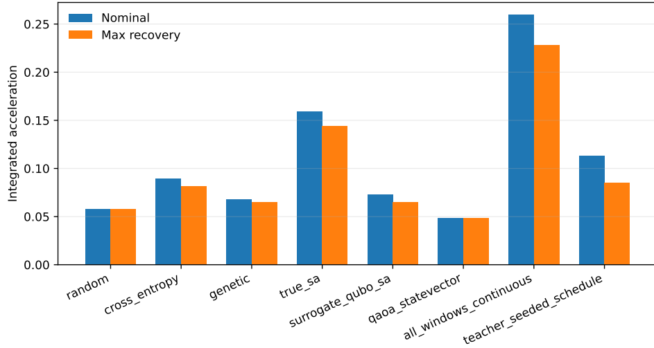
Figure 22: Teacher-controlled nominal and recovery fuel summaries. Fuel differences must be interpreted together with feasibility and missed-thrust error.
