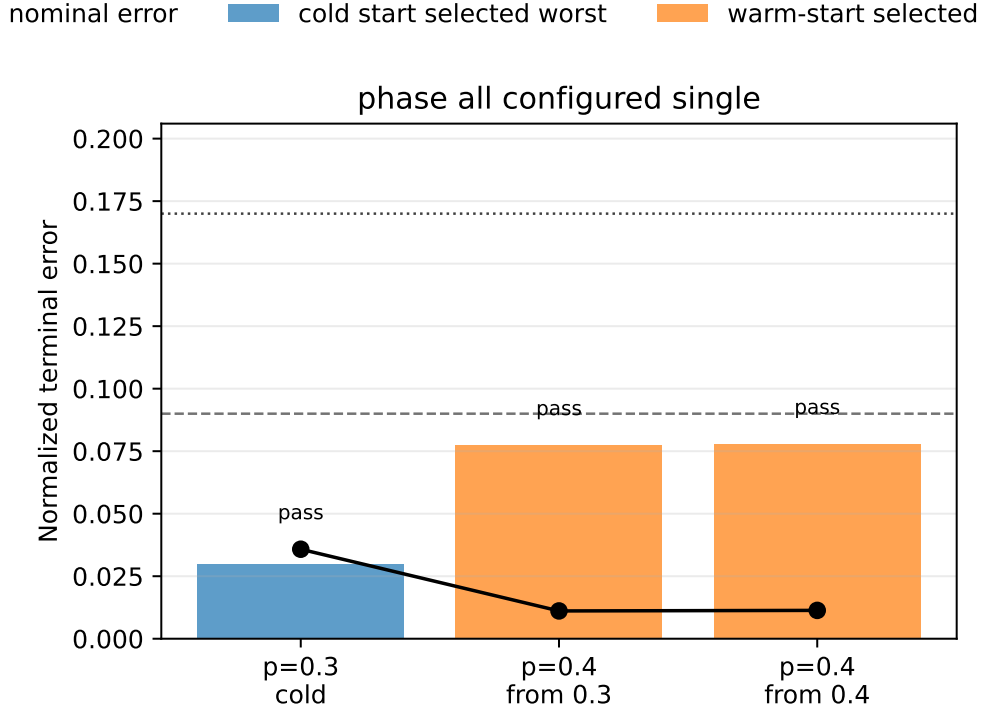
Figure 16: Independent-midpoint-control Hermite–Simpson all-configured headroom summary for the p=0.4 , a_{\max} = 0.2 phase-shift row.
