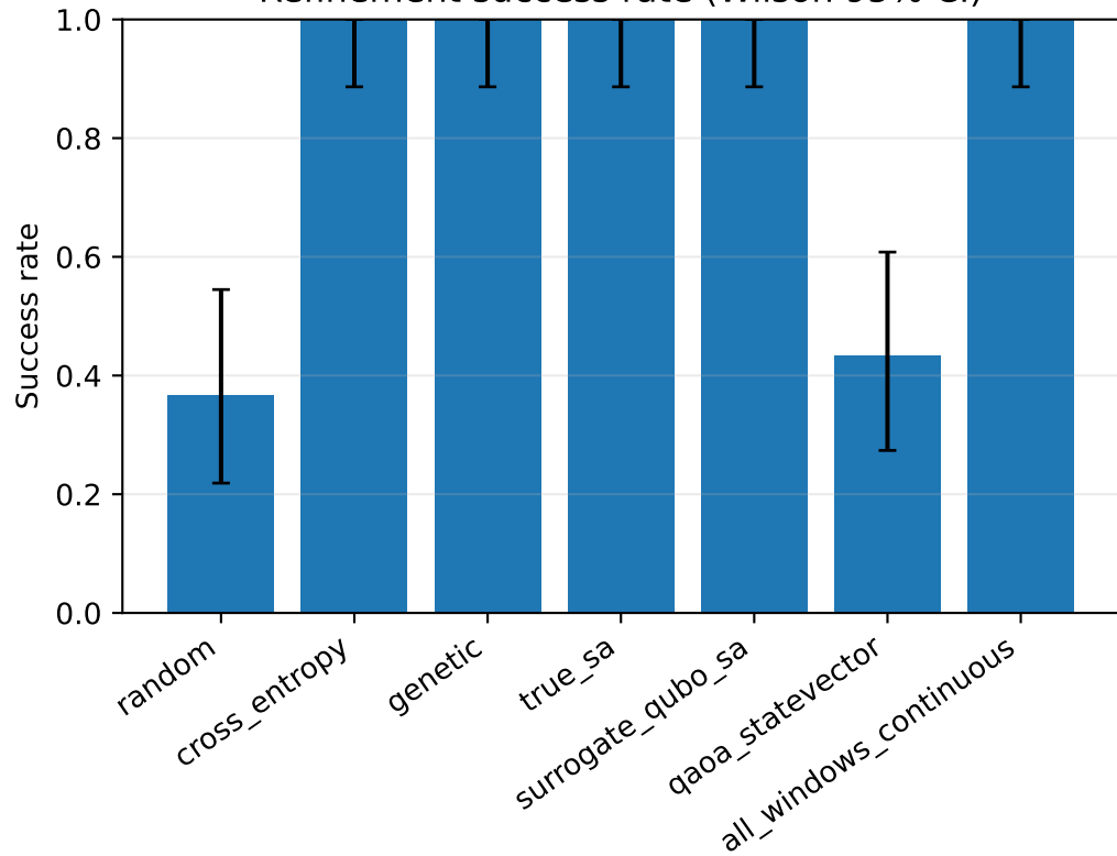
Refinement success rate (Wilson 95% CI)
