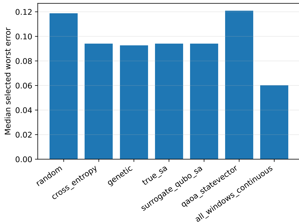
Median refined selected-worst error
