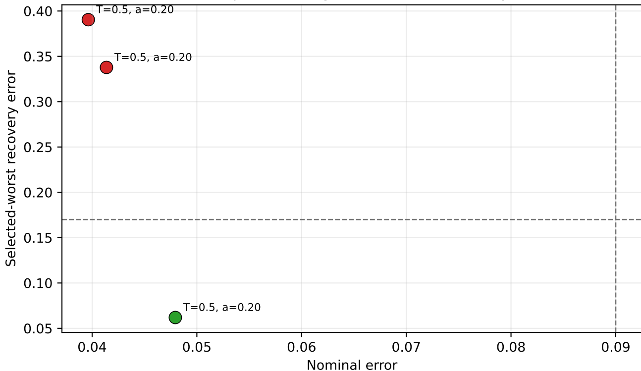
Multiple-shooting all-windows feasibility
