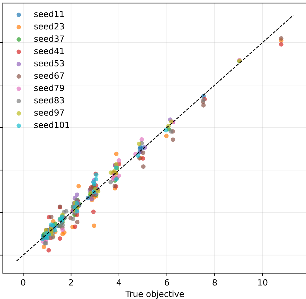
QUBO surrogate prediction
