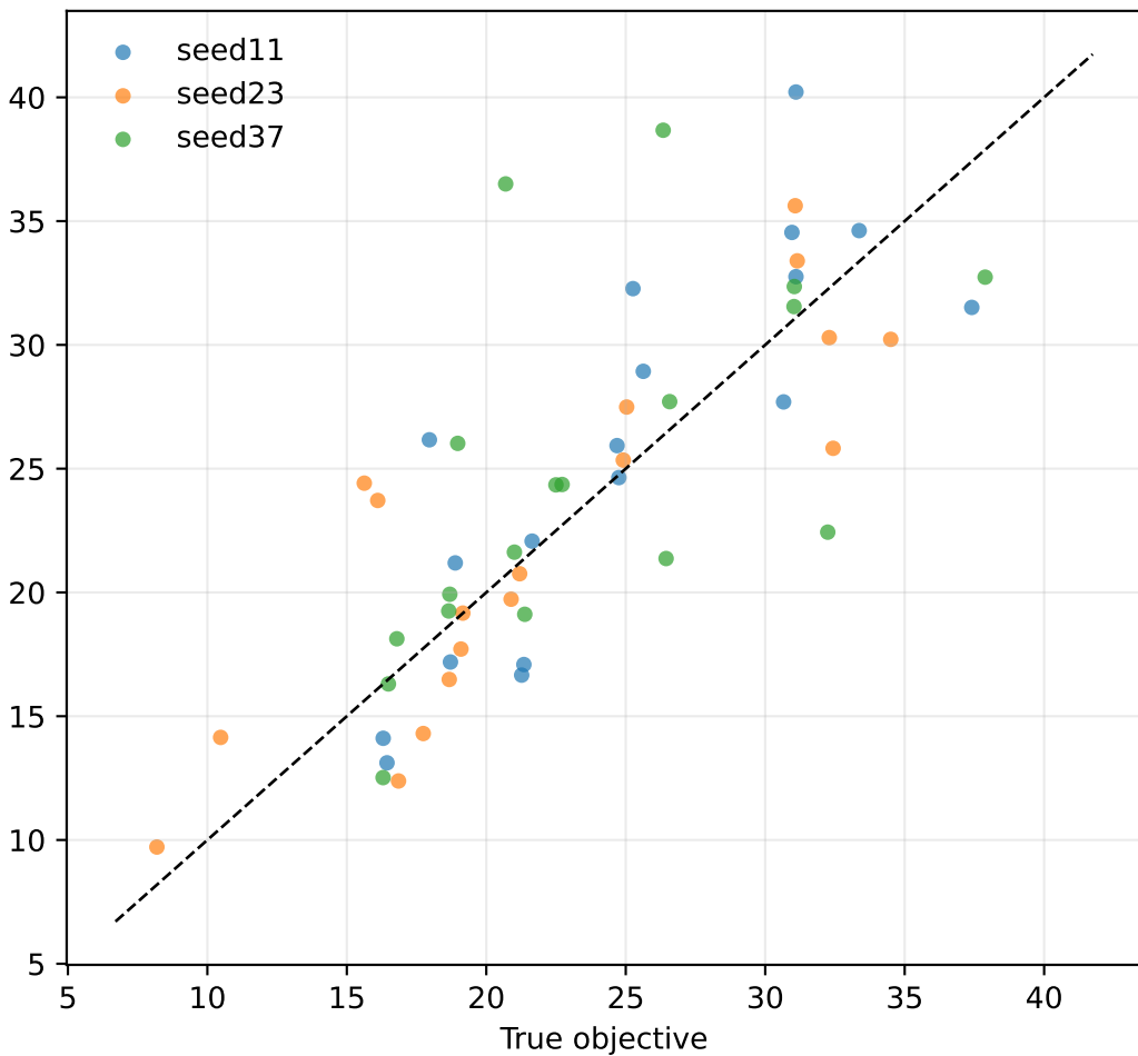
QUBO surrogate prediction
