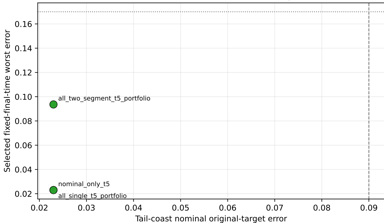
Fixed-final-time tail-coast recovery
