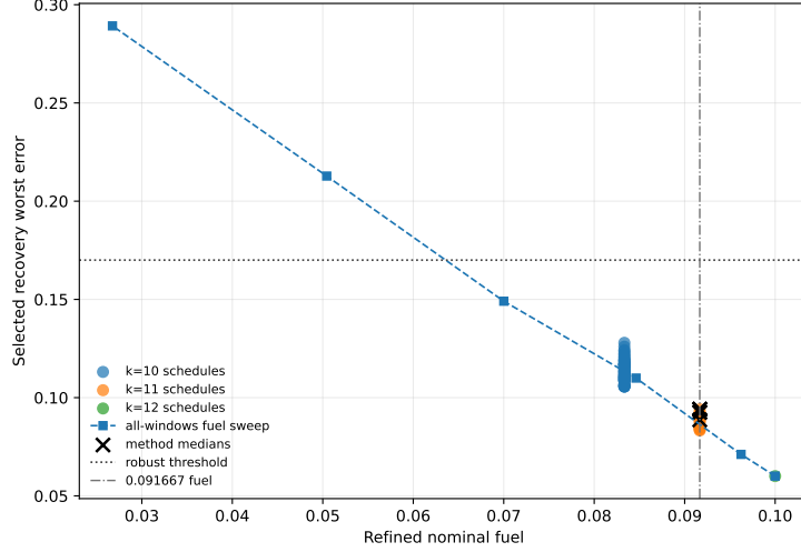
Figure 6: Fuel-error Pareto view for the duty-cycle-prior ablation. Lower fuel is achievable with all-windows fuel regularization while retaining feasibility, so the one-coast result should be read as a schedule-structure feasibility result rather than a fuel-optimality result.
