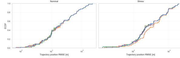
S-Figure 3: Empirical cumulative distribution of trajectory-step position error (m). On the stress split the median trajectory RMSE is about 2.51 km (AUKF), 2.47 km (RGR-GF), and 3.74 km (fixed-noise UKF), while the 90th-percentile tail remains about 11.6–13.0 km for all three, so the learned model mainly reduces fixed-noise-UKF degradation without creating a new tail-safety regime.
