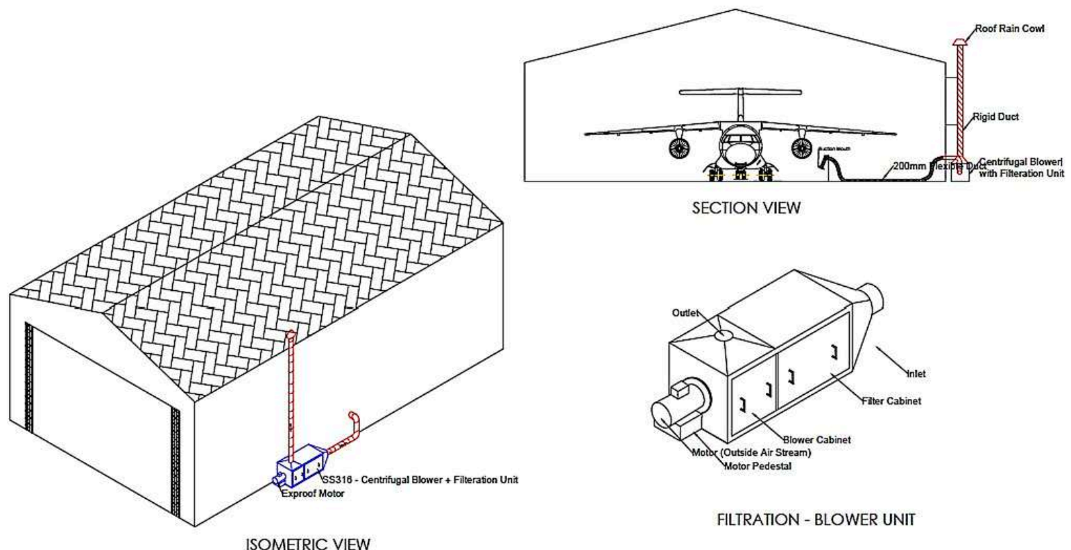
FUMES EXTRACTION SYSTEM TYPICAL DRAWING
