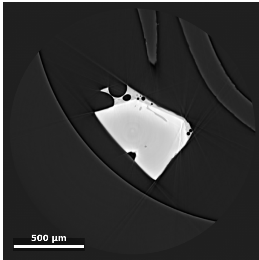
(b) Svartsengi December 2023 - Olivine
