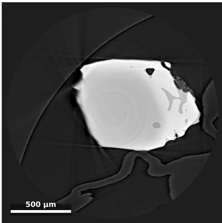
(c) Svartsengi February 2024 - Olivine
