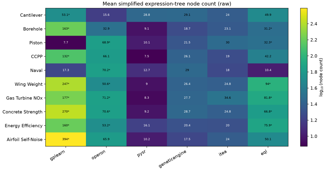
Figure 6.7: Mean simplified expression-tree node count by framework and problem using raw inputs. An asterisk indicates that at least one expression in the cell required the unsimplified complexity fallback and was excluded from the displayed simplified mean.
