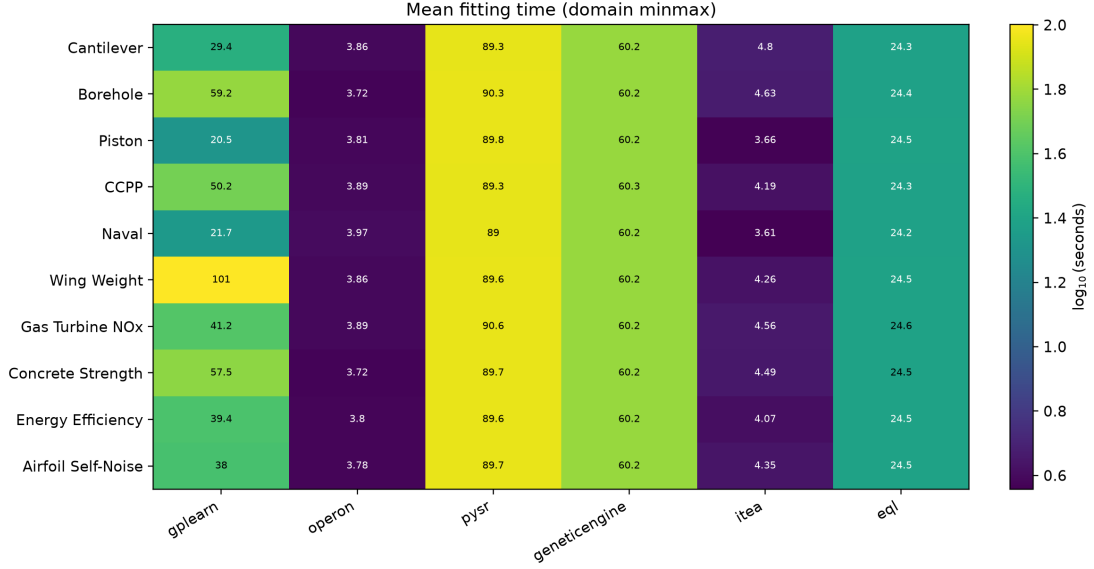
Figure 6.10: Mean model-fitting time by framework and problem using domain-normalized inputs. Cell colors represent the base-10 logarithm of time, while annotations report seconds and are based on successful trials only.
