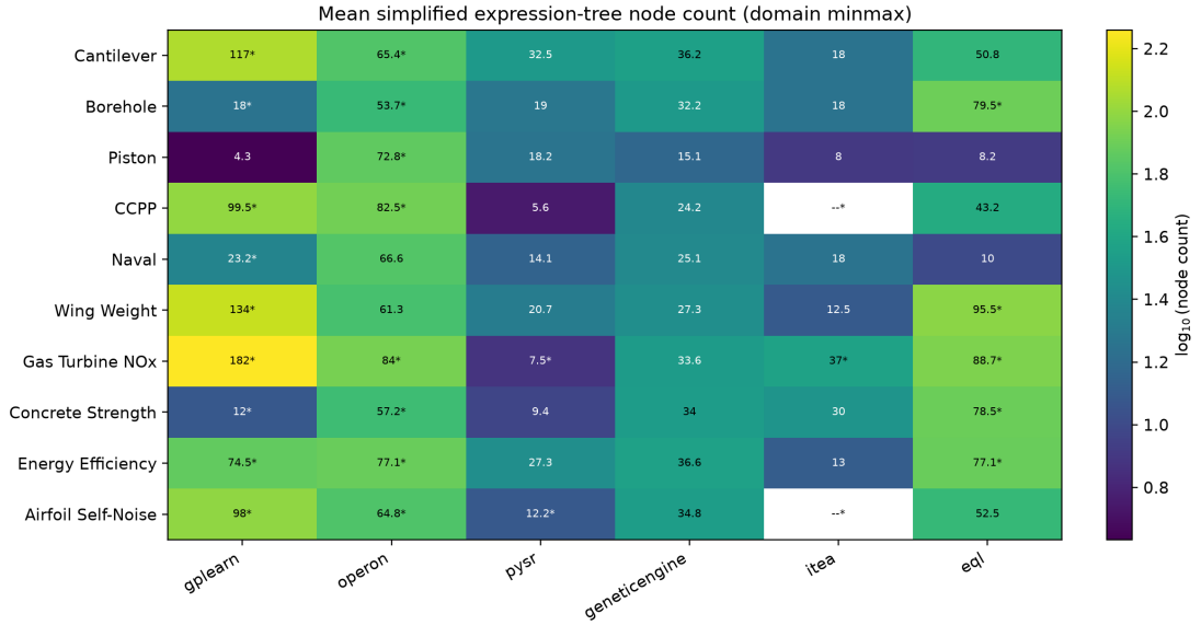
Figure 6.8: Mean simplified expression-tree node count by framework and problem using domain-normalized inputs. An asterisk indicates that at least one expression in the cell required the unsimplified complexity fallback and was excluded from the displayed simplified mean.
