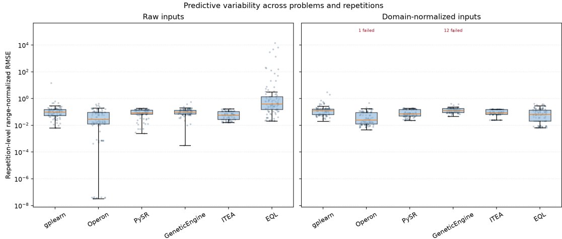
Figure 6.6: Distribution of repetition-level range-normalized RMSE by framework and input-scaling condition. Points represent successful trials across all problems, boxes summarize their distributions, and red annotations report failed trials.
