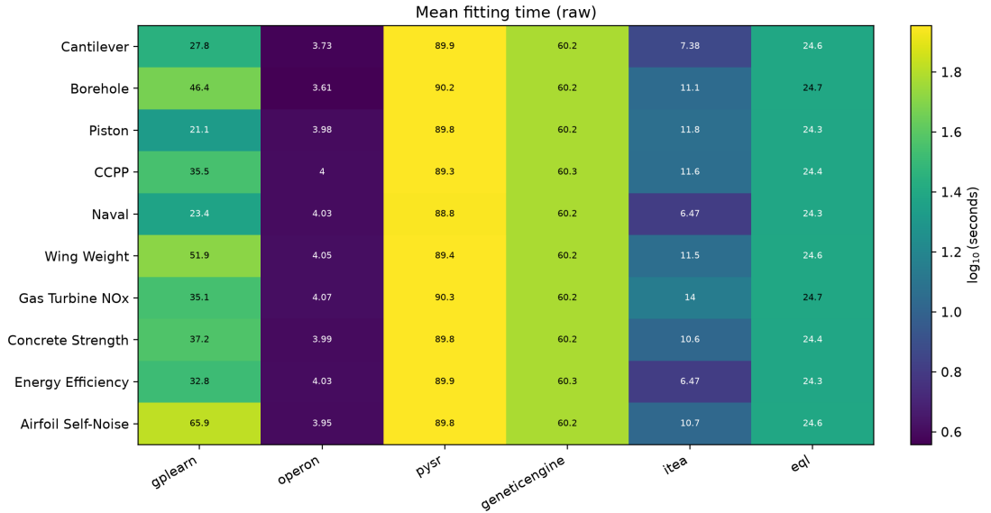
Figure 6.9: Mean model-fitting time by framework and problem using raw inputs. Cell colors represent the base-10 logarithm of time, while annotations report seconds.
