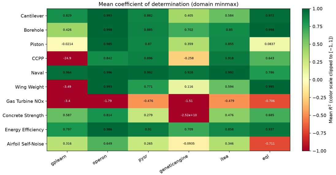
Figure 6.4: Mean coefficient of determination by framework and problem using domain-normalized inputs. The color scale is clipped to [-1, 1] , while annotations report the untruncated values.
