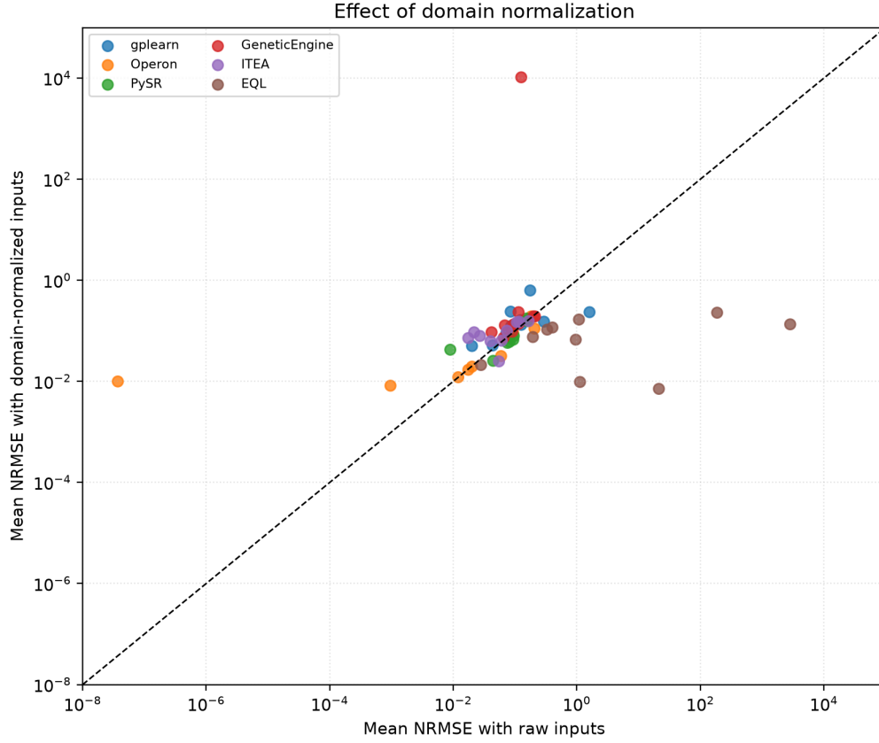
Figure 6.5: Effect of domain normalization on mean range-normalized RMSE. The diagonal represents equal error under both input-scaling conditions.
