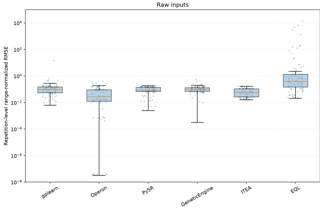
Figure 6.6: Distribution of repetition-level range-normalized RMSE by framework using raw inputs. Points represent successful trials across all problems and boxes summarize their distributions.
