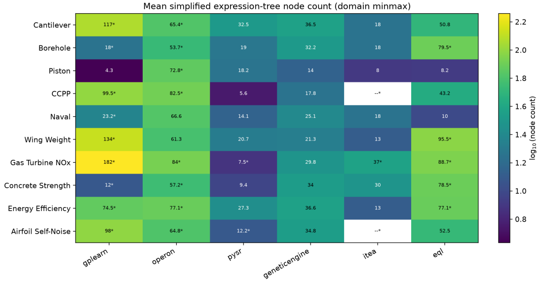
Figure 6.9: Mean simplified expression-tree node count by framework and problem using domain-normalized inputs. An asterisk indicates that at least one expression in the cell required the unsimplified complexity fallback and was excluded from the displayed simplified mean.
