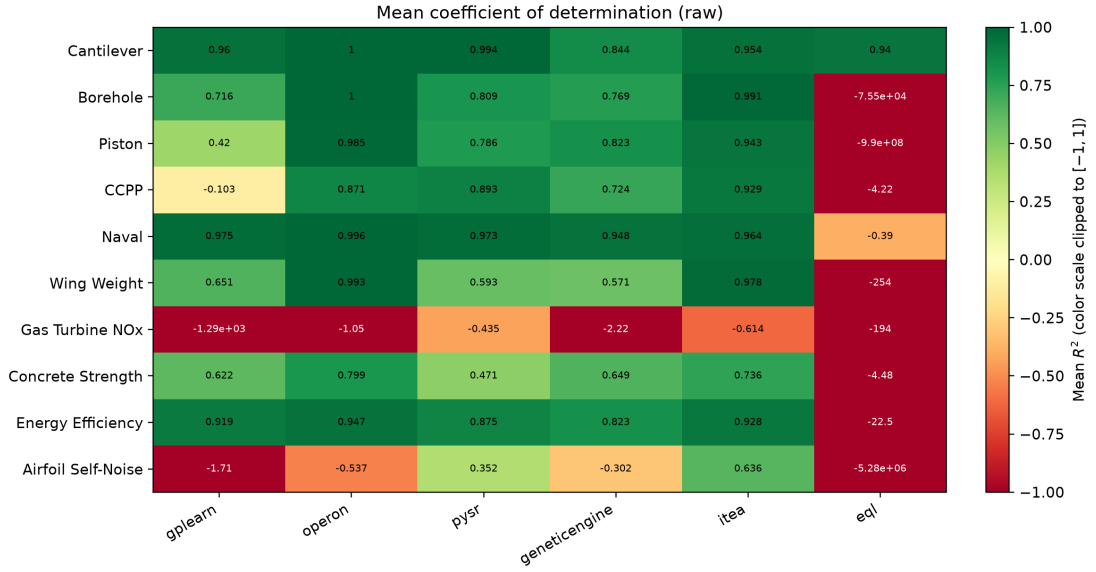
Figure 6.3: Mean coefficient of determination by framework and problem using raw inputs. The color scale is clipped to [-1, 1] , while annotations report the untruncated values.
