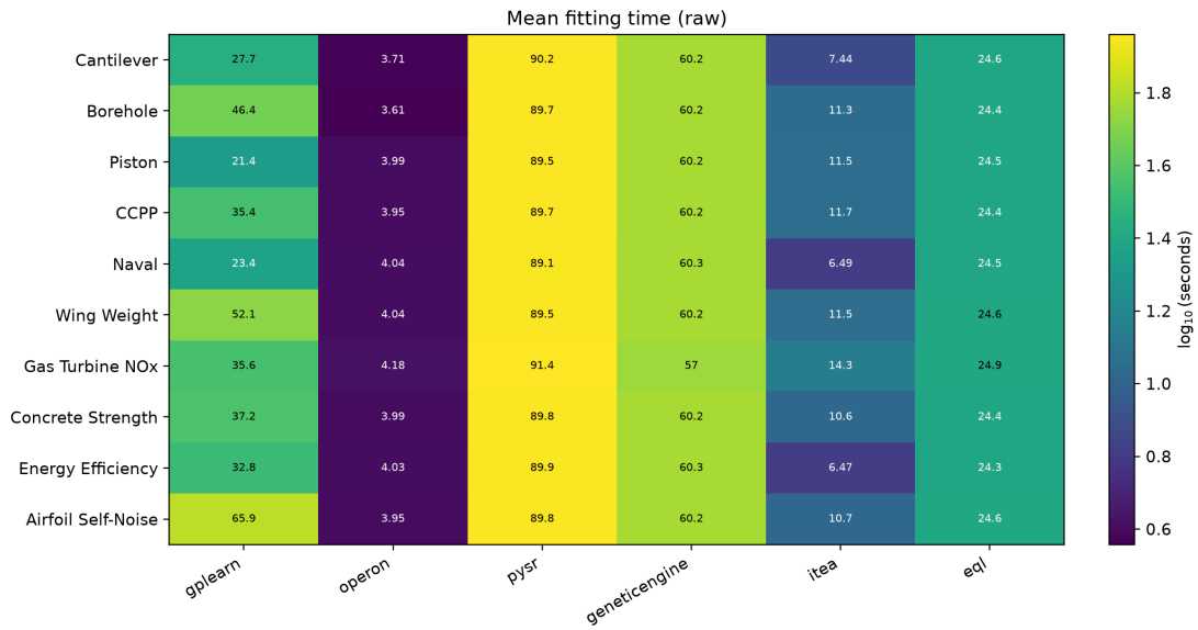
Figure 6.10: Mean model-fitting time by framework and problem using raw inputs. Cell colors represent the base-10 logarithm of time, while annotations report seconds.
