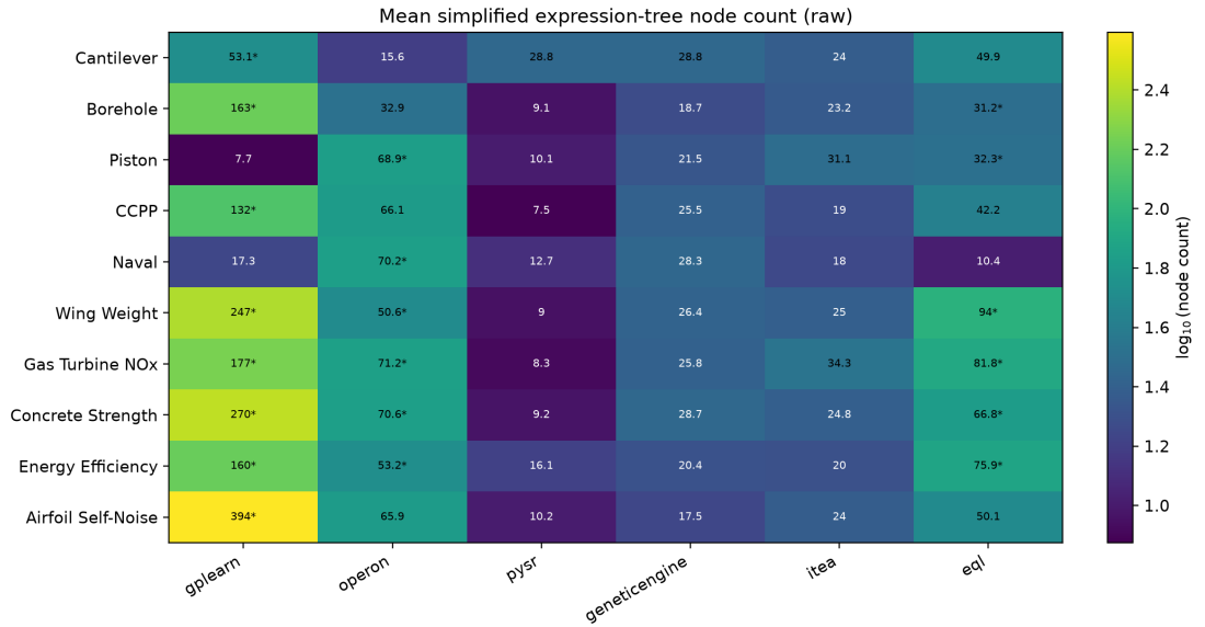
Figure 6.8: Mean simplified expression-tree node count by framework and problem using raw inputs. An asterisk indicates that at least one expression in the cell required the unsimplified complexity fallback and was excluded from the displayed simplified mean.
