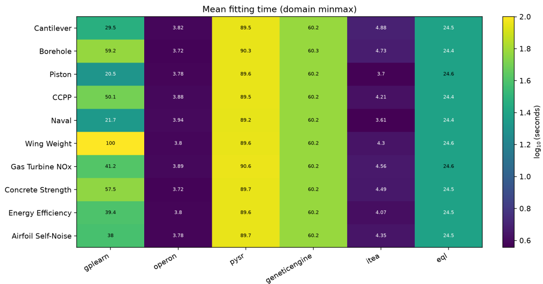
Figure 6.11: Mean model-fitting time by framework and problem using domain-normalized inputs. Cell colors represent the base-10 logarithm of time, while annotations report seconds and are based on successful trials only.
