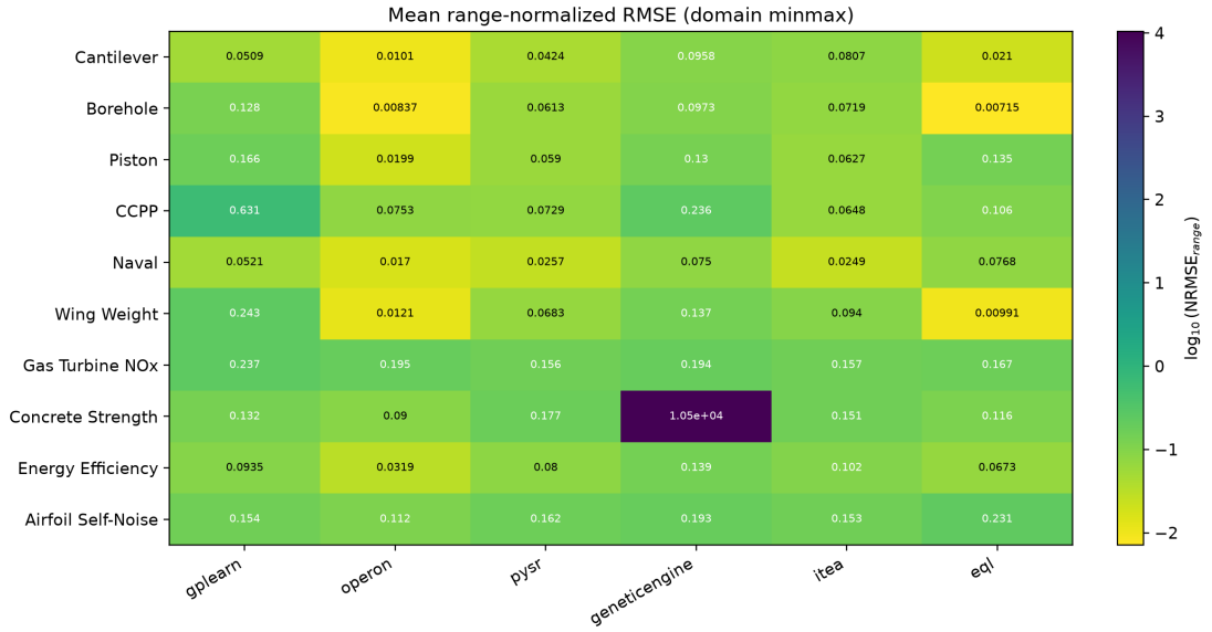
Figure 6.2: Mean range-normalized RMSE by framework and problem using domain-normalized inputs. Cell colors represent the base-10 logarithm of NRMSE, while annotations show the untransformed values.
