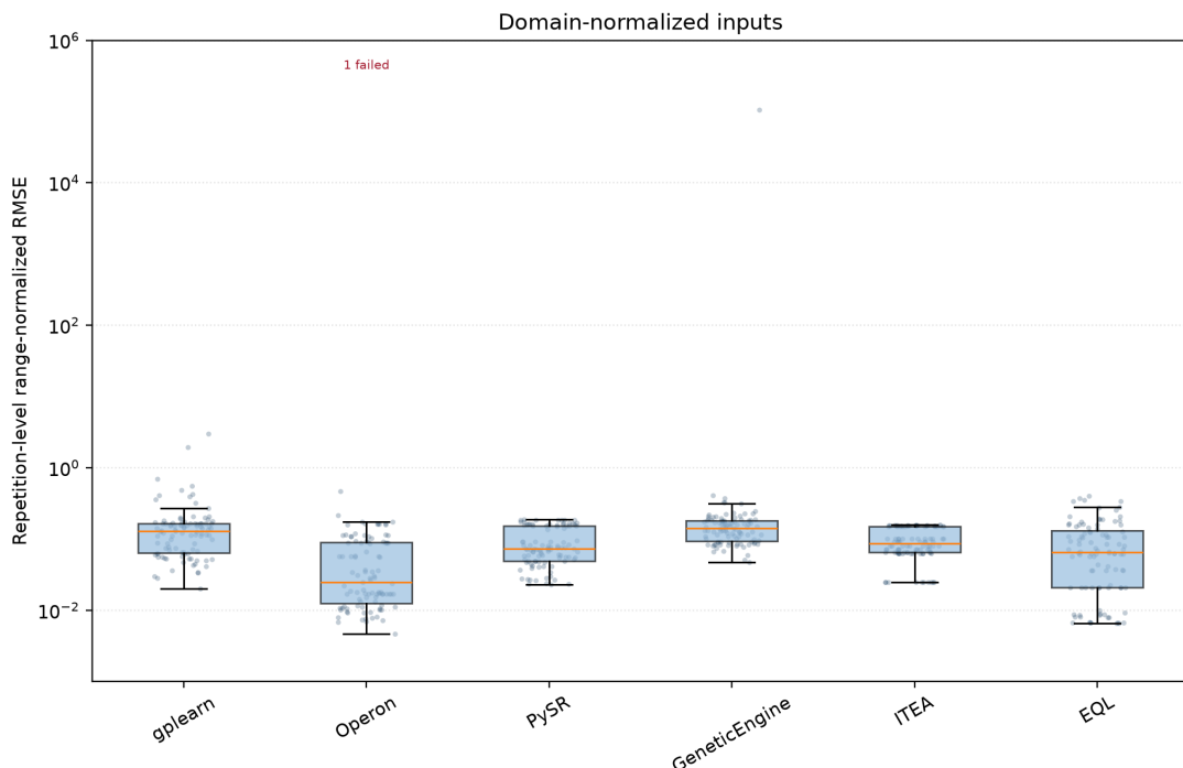
Figure 6.7: Distribution of repetition-level range-normalized RMSE by framework using domain-normalized inputs. Points represent successful trials across all problems, boxes summarize their distributions, and red annotations report failed trials.
