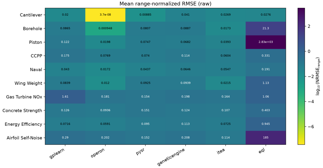
Figure 6.1: Mean range-normalized RMSE by framework and problem using raw inputs. Cell colors represent the base-10 logarithm of NRMSE, while annotations show the untransformed values.
