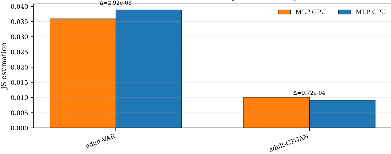
Use case 11: MLP GPU vs MLP CPU JS estimation, train_100
