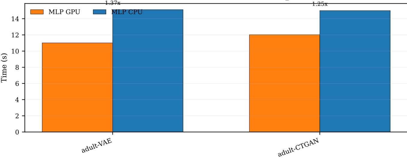
Use case 11: MLP GPU vs MLP CPU time, train_100
