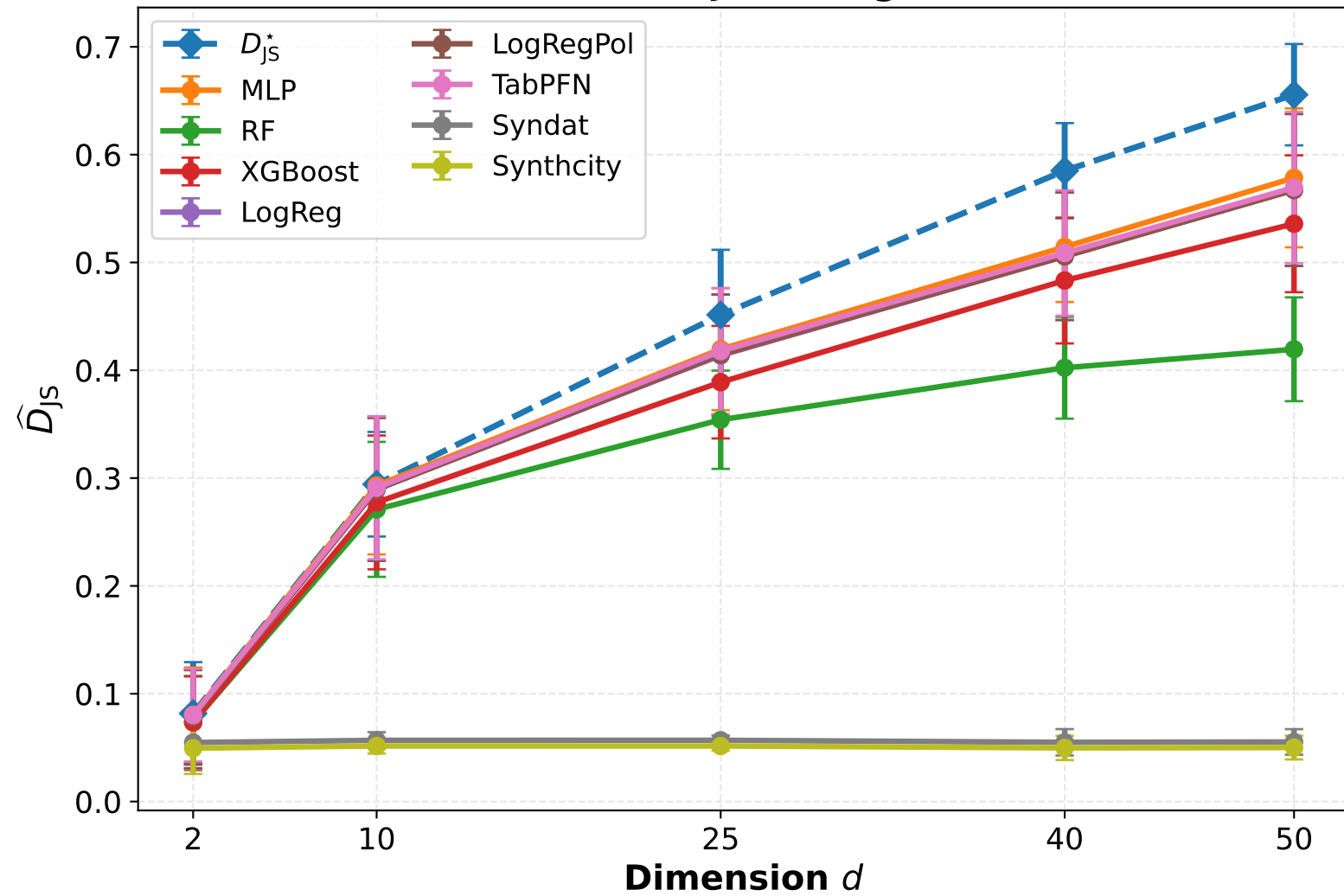
Estimated JS divergence
