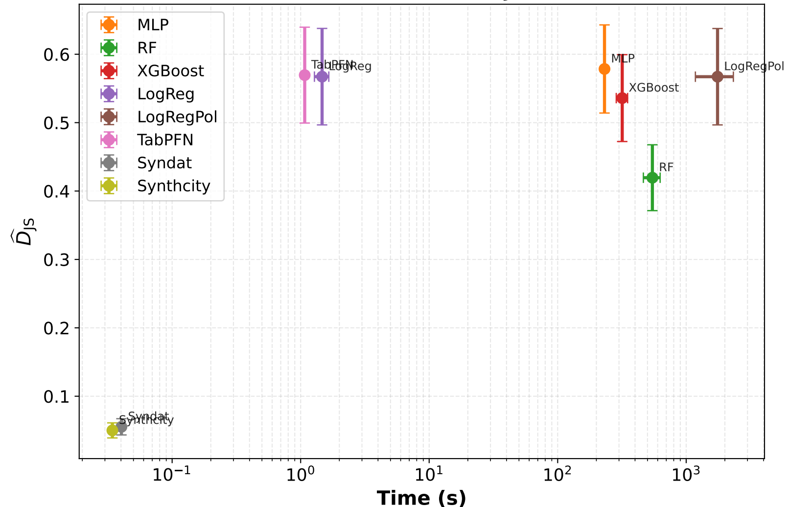
Runtime vs estimated JS, d=50
