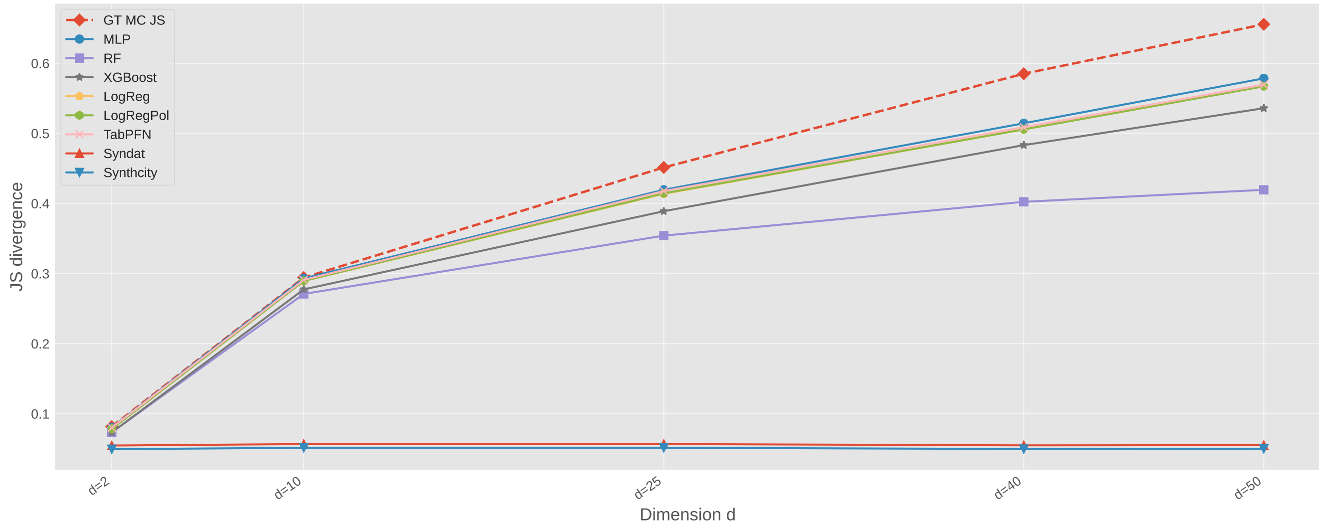
JS divergence across dimensions (UC7)
