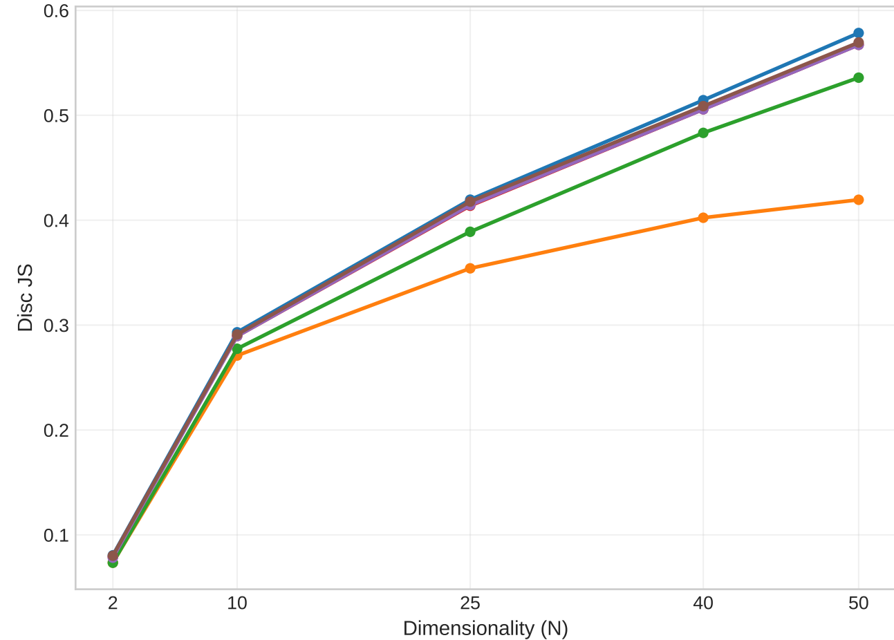
UC7 JS by dimensionality
