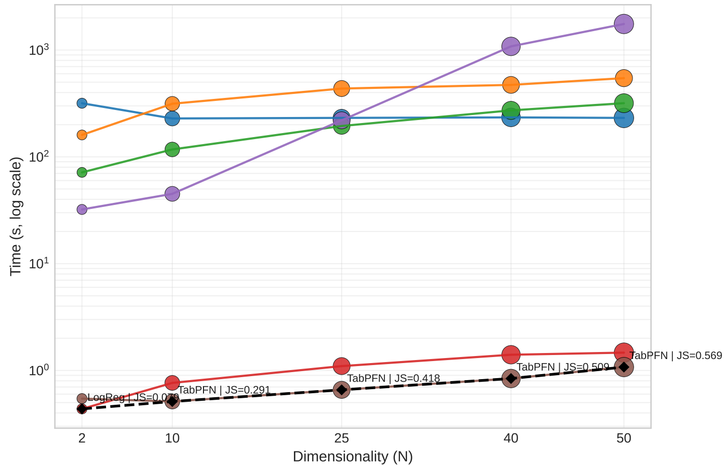
UC7 Pareto: time vs dimensionality
