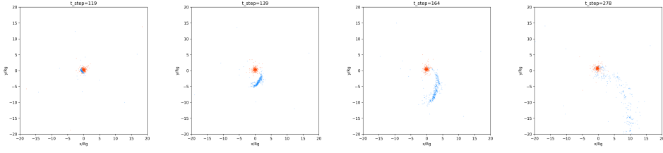
Figure 2: Evolution of the flyby of a lower mass galaxy next to a Milky-Way sized galaxy.
