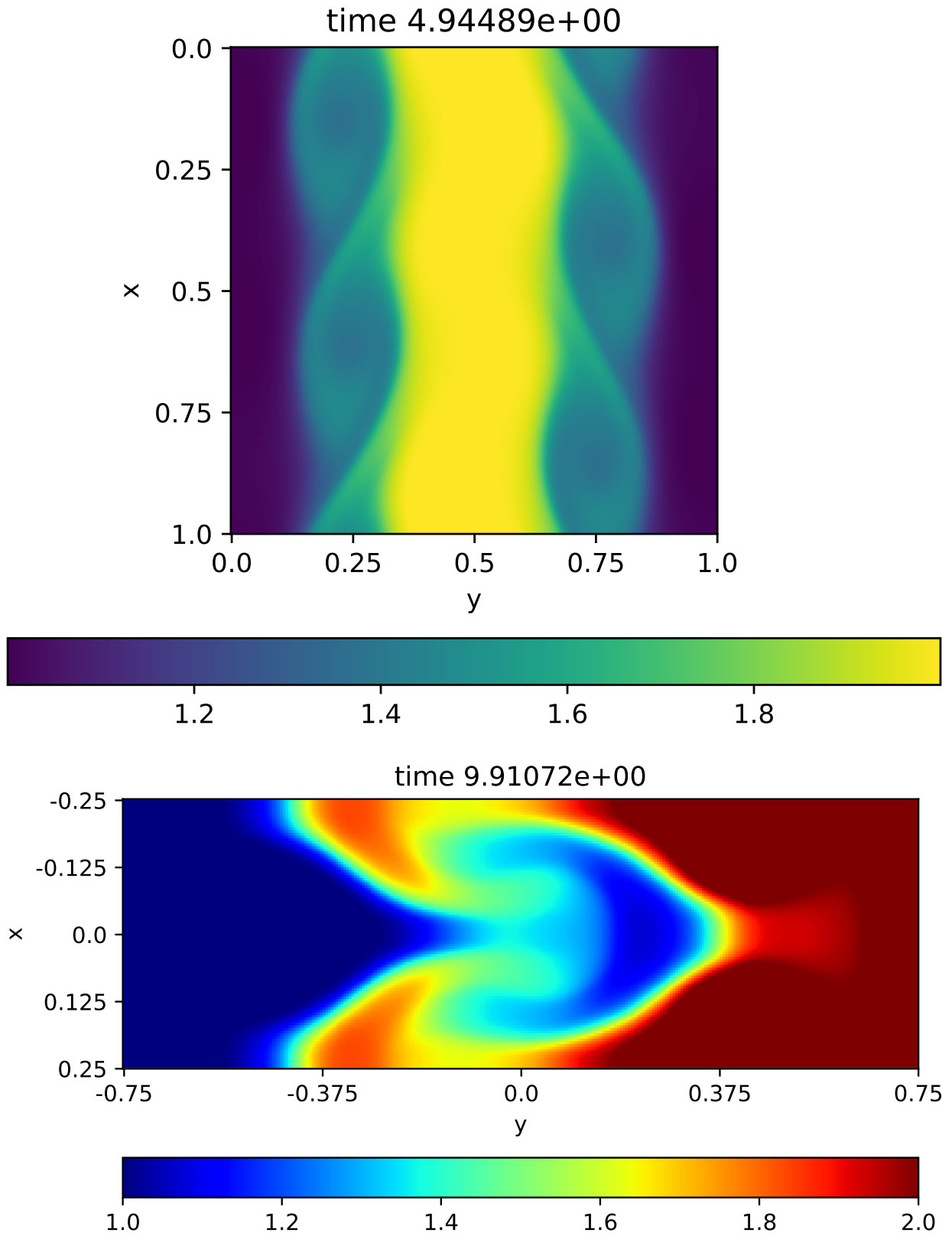
Figure 5: Top: Kelvin-Helmholtz instability after nearly 5s, with a 256 by 256 resolution. Bottom: Rayleigh-Taylor instability after nearly 10s, with a 100 by 300 resolution. The structures which should form smeared into much more diffuse elements.
