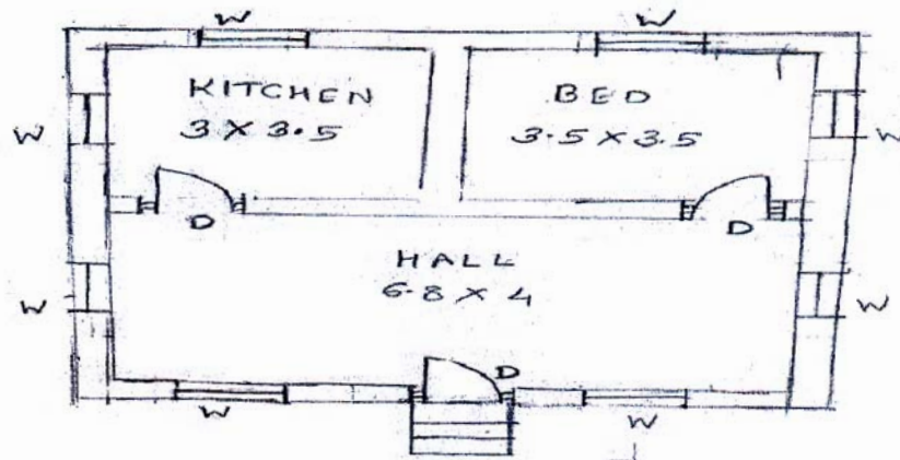
Fig 1(A) PLAN
