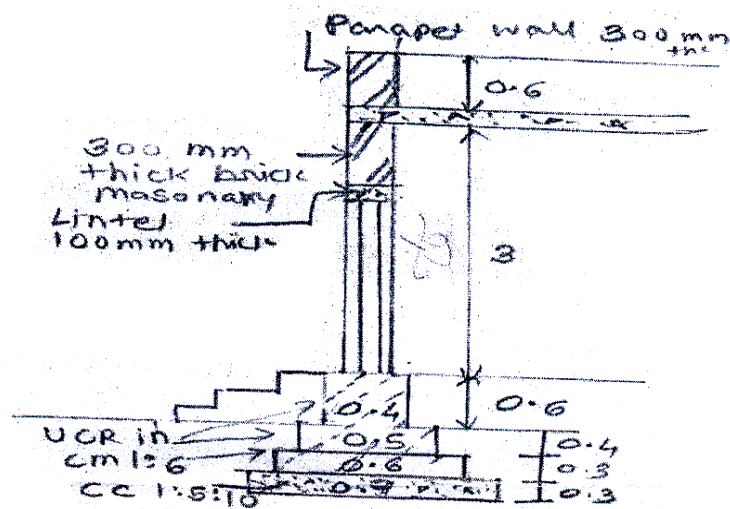
Fig 1(B) ELEVATION
