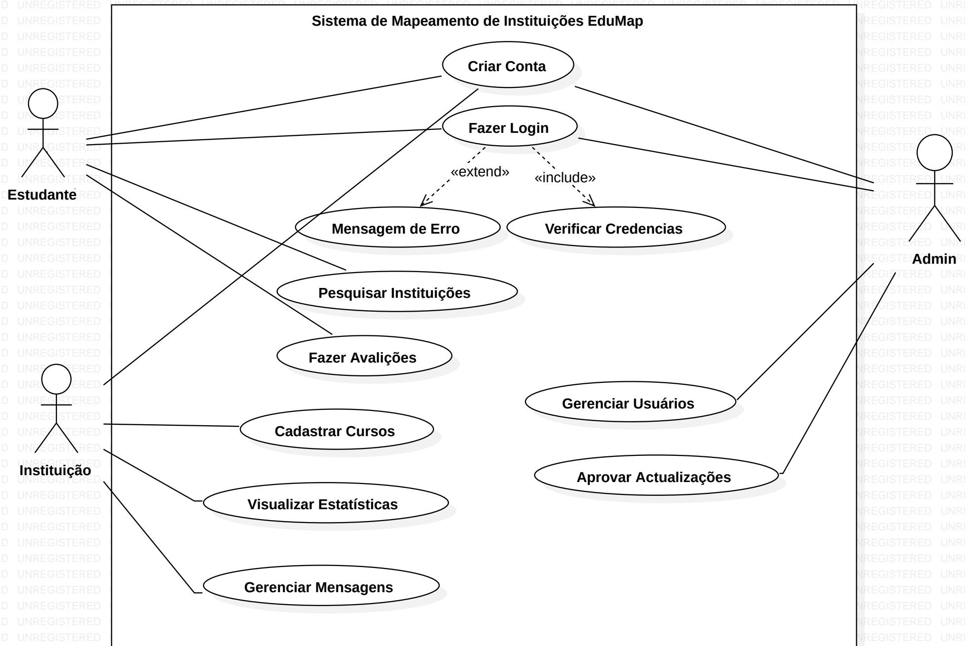
Model1::UseCaseDiagram1
