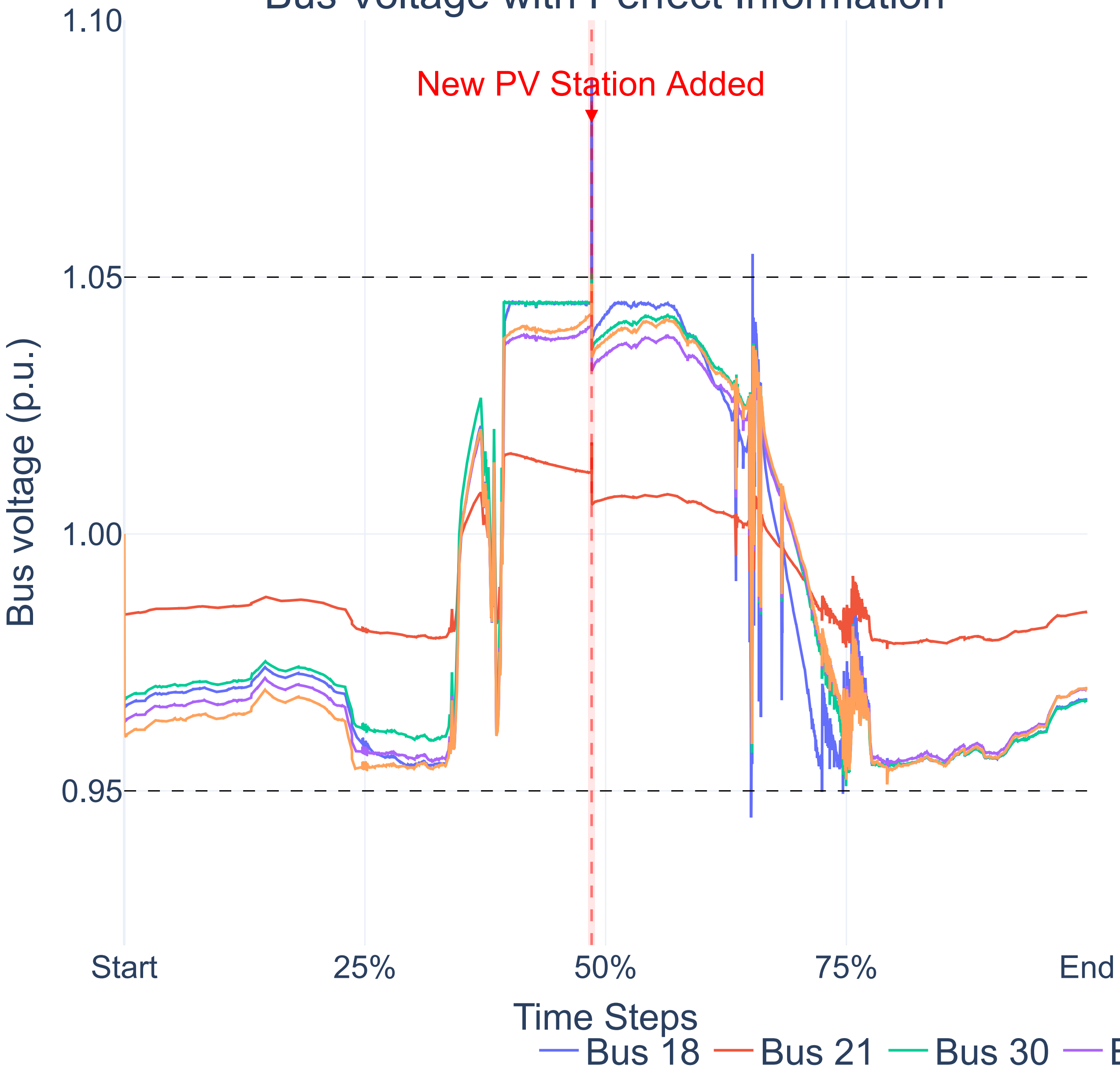
Bus Voltage with Perfect Information
