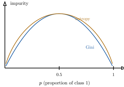
Figure 3: Gini impurity and entropy for a two-class node, against the proportion p of one class. Both are zero at the pure ends ( p = 0 or 1 ) and peak at the even mixture p = 0.5 . They have the same shape, so the splitting criterion almost never changes which tree you get; entropy is marginally costlier to compute because of the logarithm.
