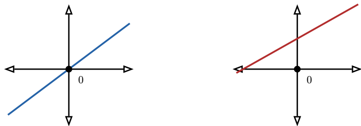
Figure 2: Every subspace contains the zero vector, so in \mathbb{R}^2 the only subspaces are \{0\} , lines through the origin , and the whole plane. A line that misses the origin (right) fails criterion 1 immediately — a quick first test before checking closure.
