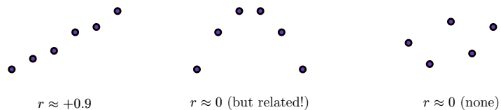
Figure 4: Correlation measures linear association only. The middle cloud has a strong relationship that correlation reports as zero — which is why a matrix is never read without scatter plots.
