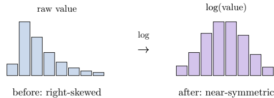
Figure 5: A log transformation pulls in a long right tail, turning a skewed distribution into a roughly symmetric one — easier to plot, summarise, and relate linearly to other variables.
