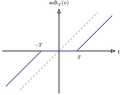
Figure 6: Soft thresholding with threshold T = \eta\lambda . Inputs in [-T, T] are snapped to exactly zero (the flat segment); larger inputs are kept but shrunk toward zero by T . The dead zone around the origin is what makes \ell_1 regularization produce sparse solutions — small coefficients are eliminated outright rather than merely shrunk.
