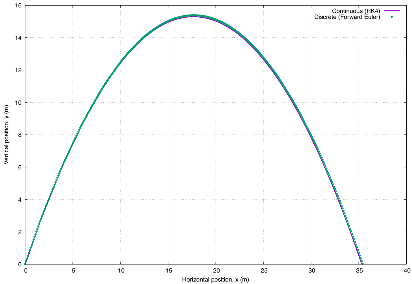
Ball Trajectory: Continuous and Discrete Models
