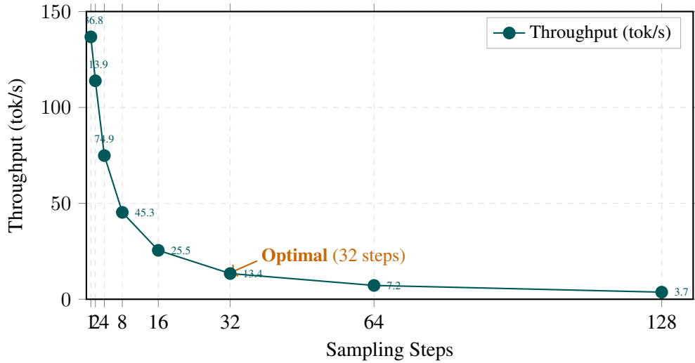
Figure 5: Token throughput (tok/s) vs. sampling steps. The curve is concave because fixed per-step overhead (CUDA kernel launches, block scheduling, sampling bookkeeping) dominates at very low step counts, making each additional step reduction yield diminishing absolute latency savings. The 32-step operating point (orange) delivers 13.4 tok/s—a 3.6\times improvement over the 128-step Teacher—while retaining the highest measured Promptfoo pass rate.
