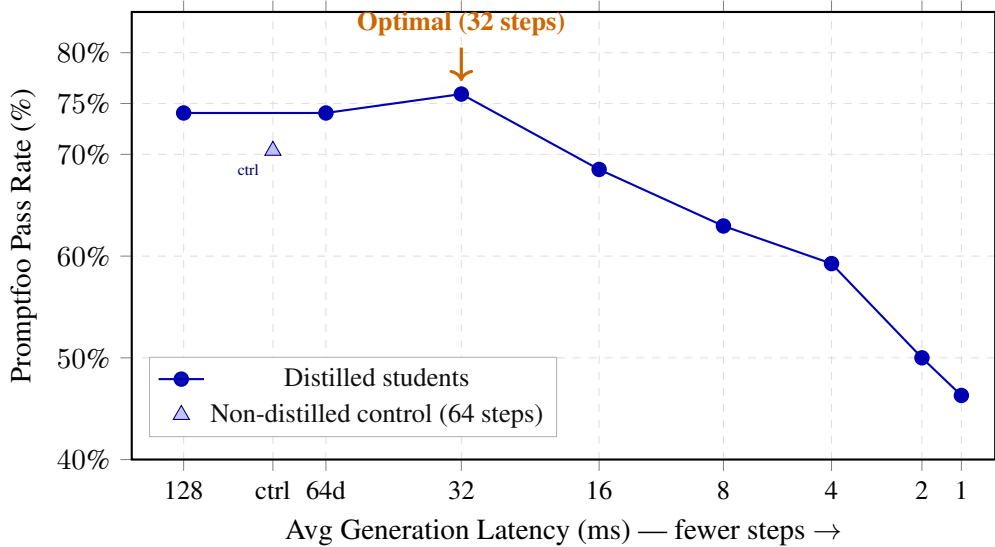
Figure 6: Generation latency vs. Promptfoo pass rate, with latency axis reversed so that faster (fewer-step) models appear on the right. Each x-tick label shows the step count for the corresponding distilled student. The 32-step student achieves the highest pass rate (75.93%), surpassing even the 128-step Teacher (74.07%) while running 3.63\times faster. Quality degrades sharply to the right of the 16-step point.
