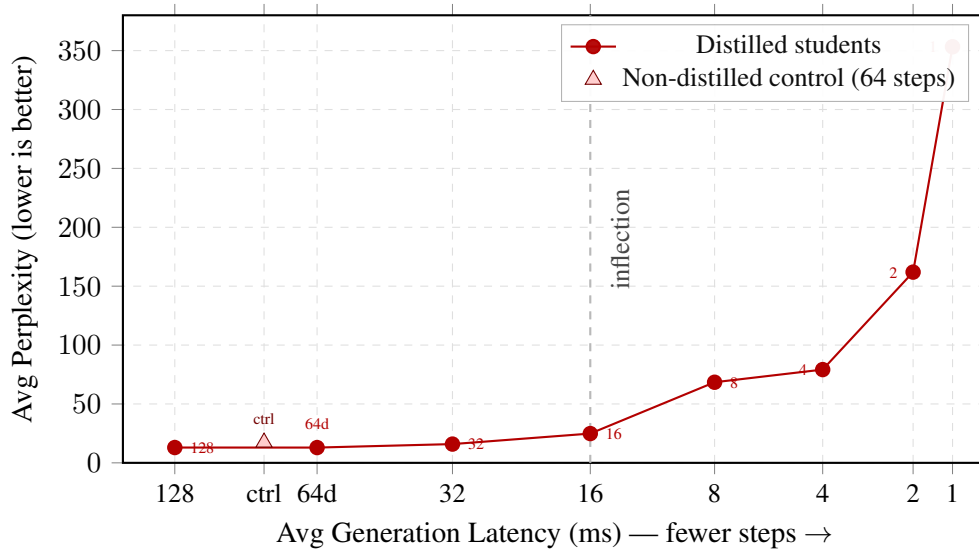
Figure 7: Generation latency vs. GPT-2 perplexity, with latency axis reversed (fewer steps on the right). Perplexity remains near the Teacher baseline from 128 down to 32 steps (15.93), then rises sharply below 16 steps, reaching 353 at a single step. The dashed vertical line marks the inflection point between the two quality regimes.
