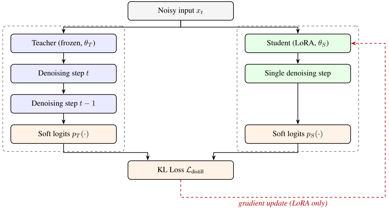
Figure 3: Knowledge Distillation Architecture
