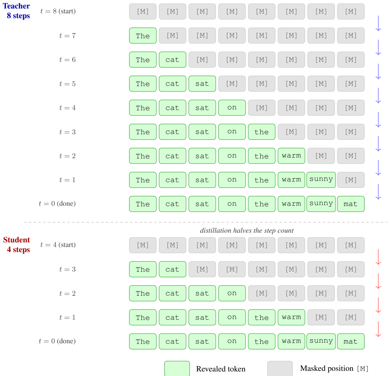
Figure 4: Token unmasking step-by-step for the sentence “ The cat sat on the warm sunny mat ”. Top (blue, Teacher, 8 steps): one token is committed per step, giving fine-grained, gradual unmasking. Bottom (red, Student, 4 steps): two tokens are committed per step. The Student is trained via KL divergence to match the Teacher’s two-step soft distributions in a single forward pass, so the tokens revealed at each distilled step are of comparable quality to those revealed after two Teacher steps—progressive distillation learns a compressed unmasking policy, not a naive step-skip.
