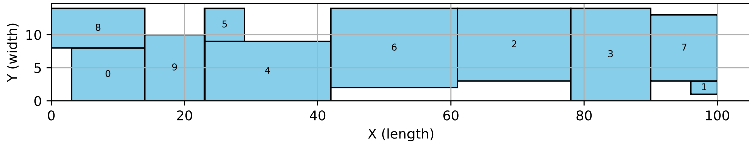
10_10 | traditional | bigm
