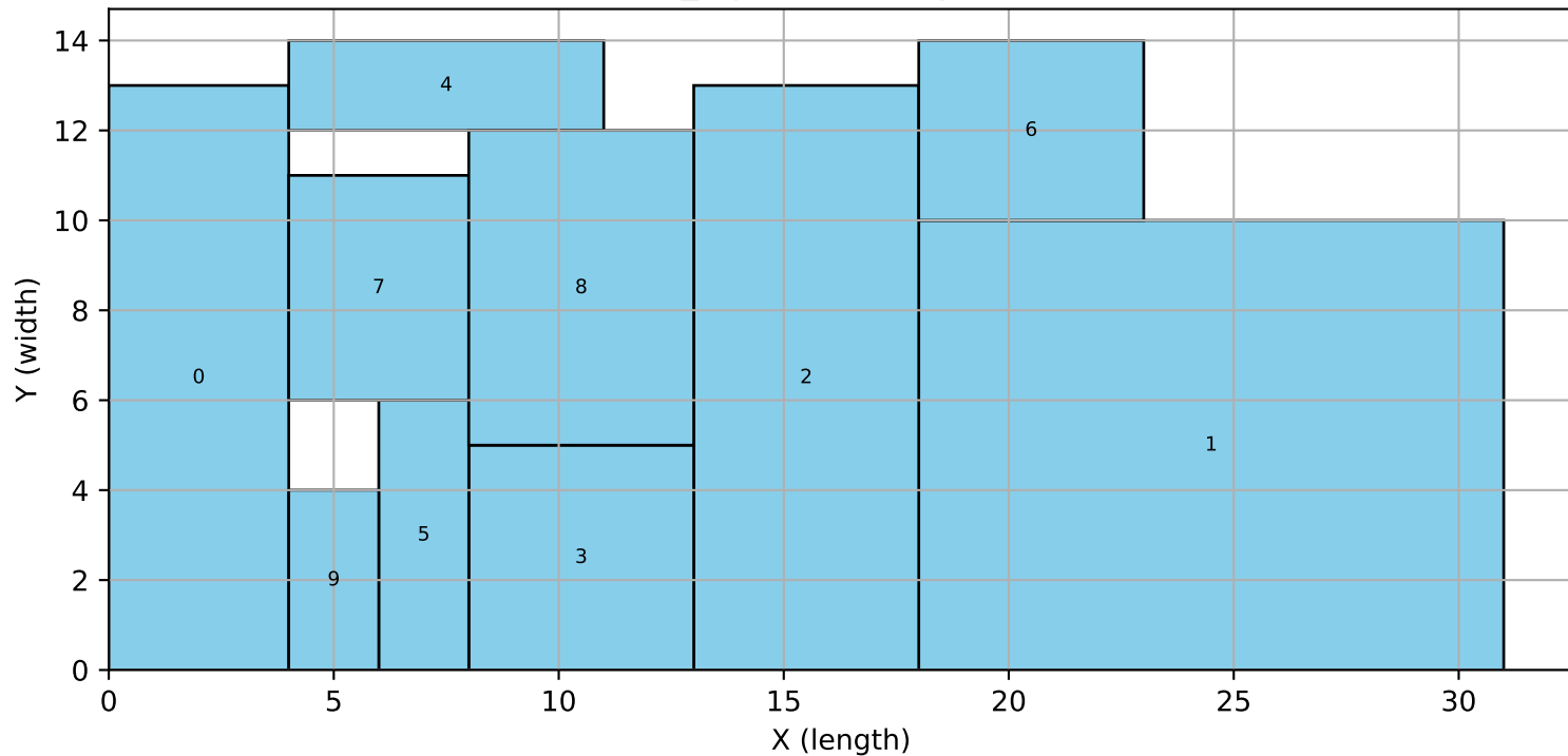
10_2 | traditional | bigm
