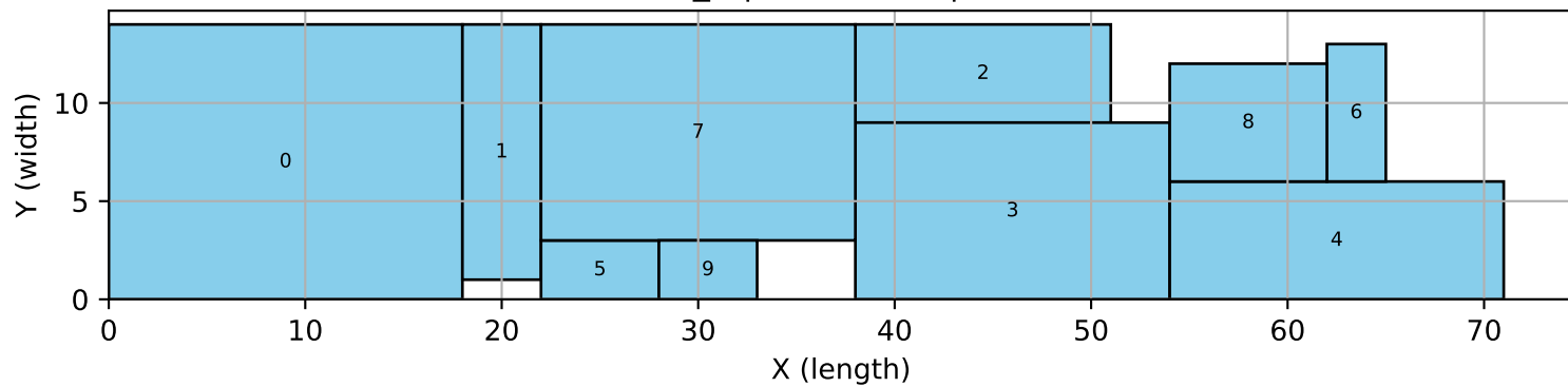
10_9 | traditional | hull
