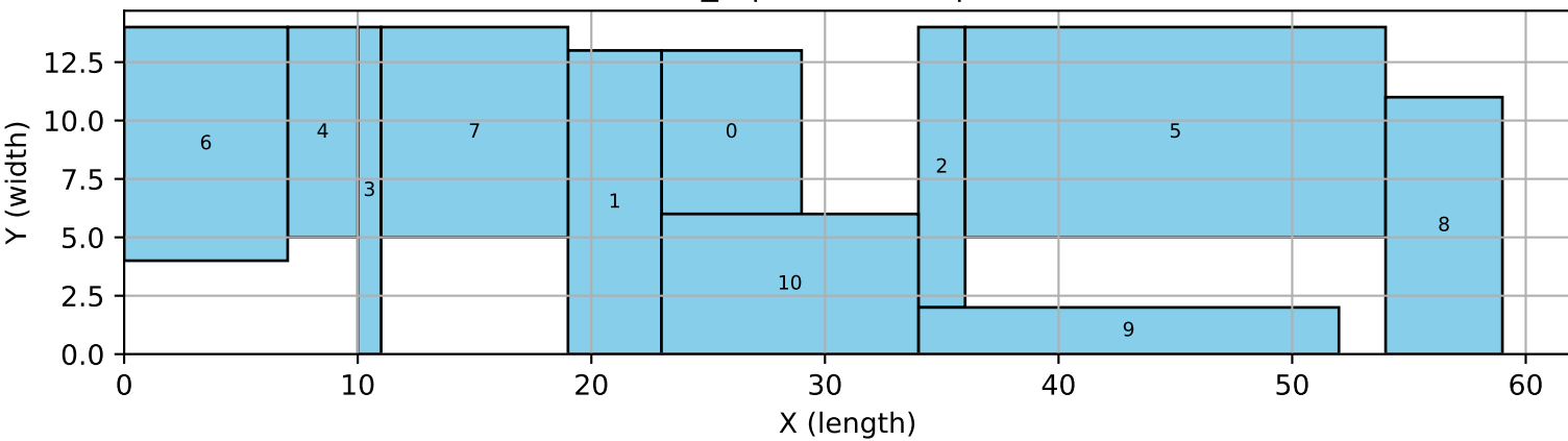
11_6 | traditional | hull
