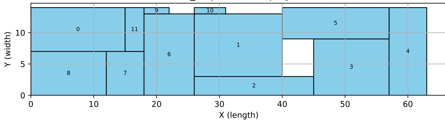
12_10 | traditional | bigm
