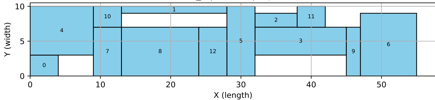
13_2 | altered | bigm
