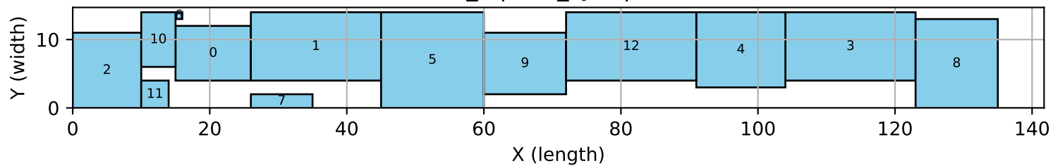
13_6 | tres_sym | hull
