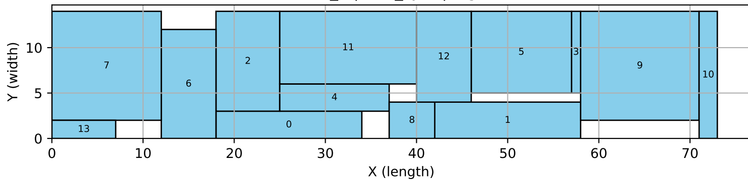
14_4 | tres_sym | bigm
