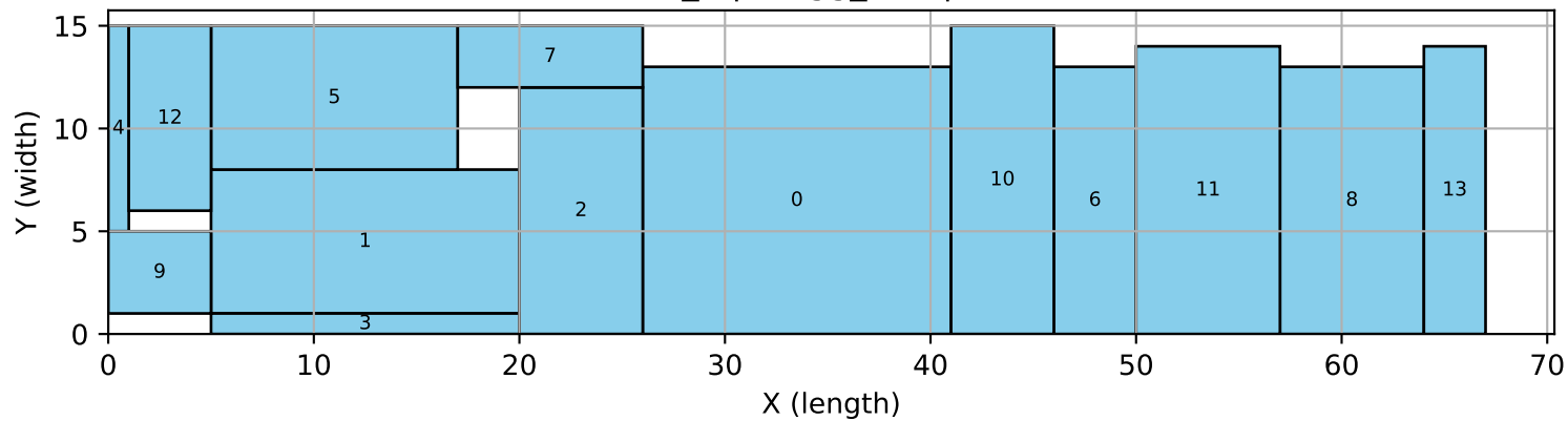
14_5 | reagg_tres | MIP
