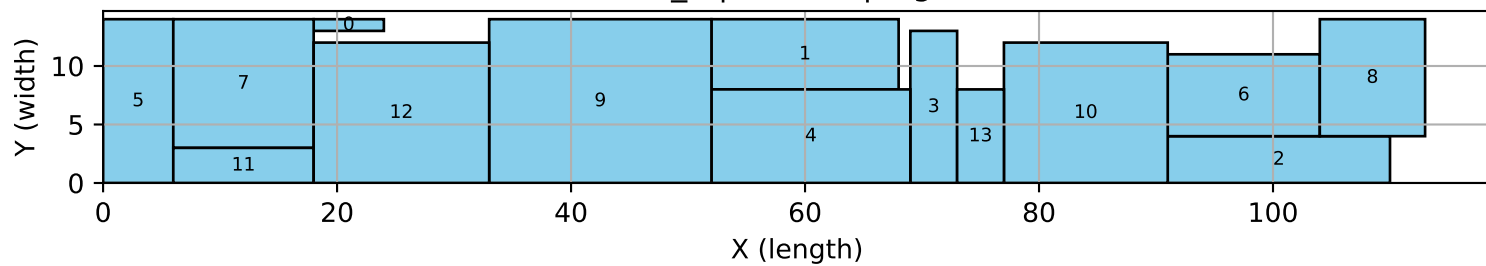
14_6 | altered | bigm
