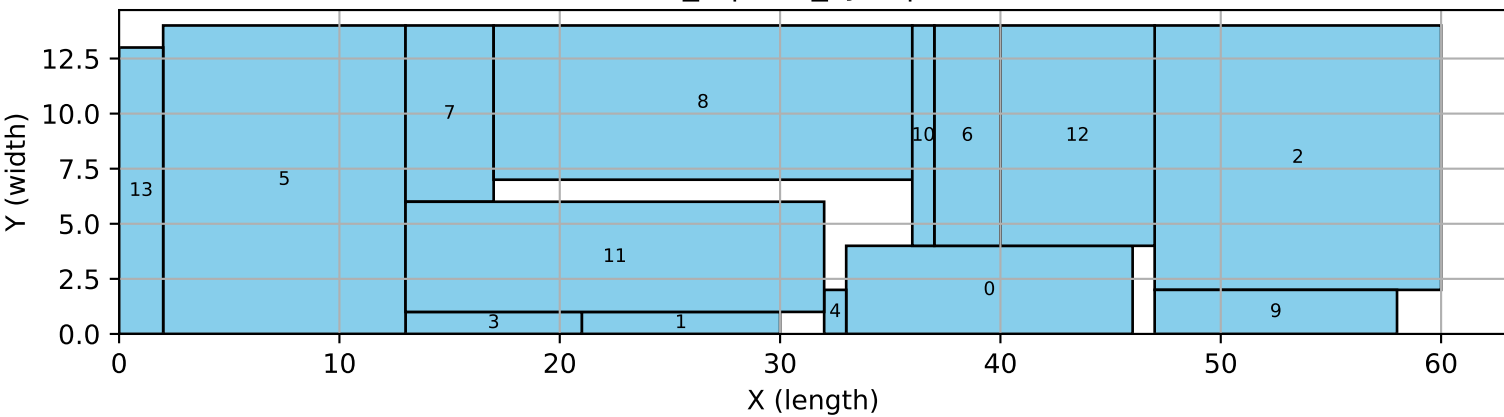
14_7 | tres_sym | hull
