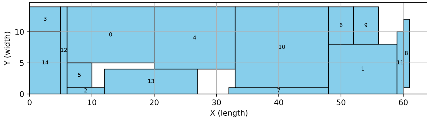
15_4 | altered | bigm
