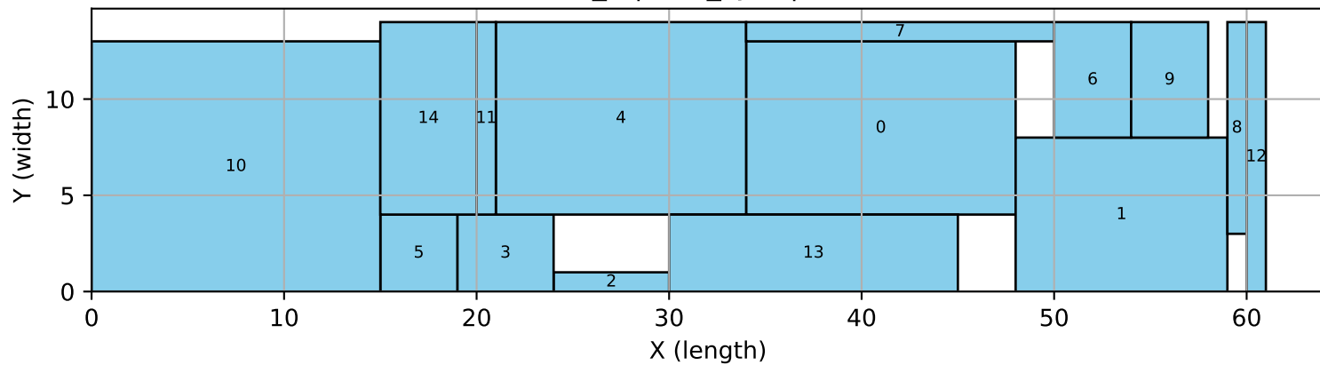
15_4 | tres_sym | hull
